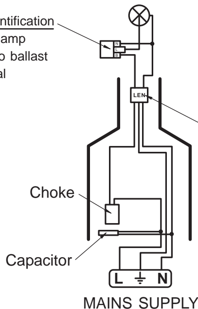
Wiring diagram for remote gear option
