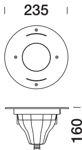
NETTUNO recessed
